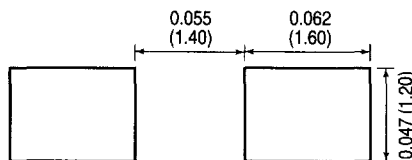
Mounting Pad Layout
